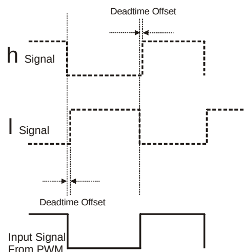
Preventing Half-Bridge Short Circuits At Switch-on With Deadtime.
