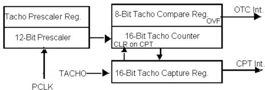
Tacho Generator Interface.
