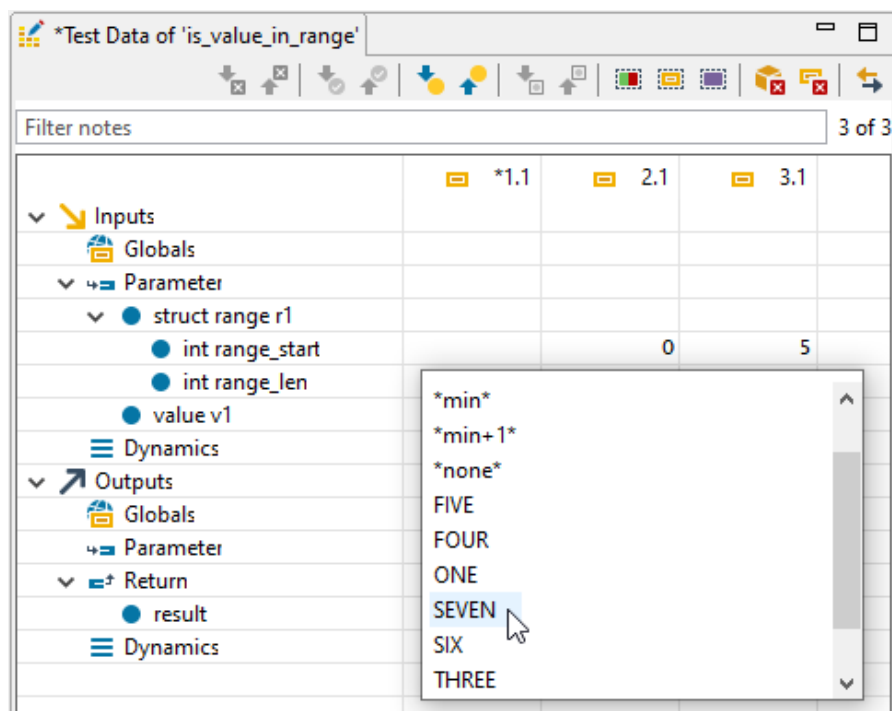
Figure 6.212: Pressing Ctrl + Space opens a list of available defines or enum constants
