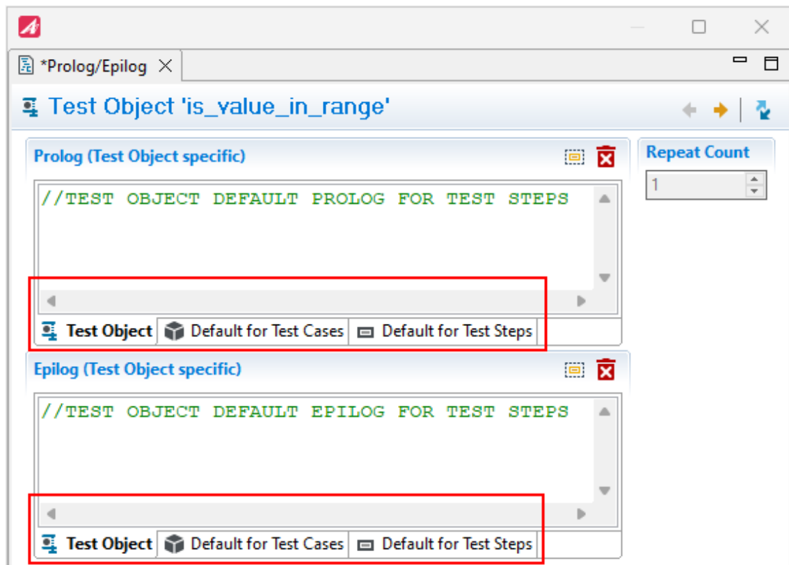
Figure 6.228: TESSY provides default prolog/epilog on test object level to be inherited to test cases and test steps
