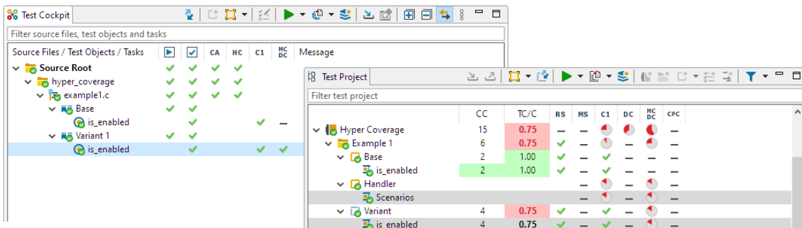
Figure 0.5: Hyper Coverage example
