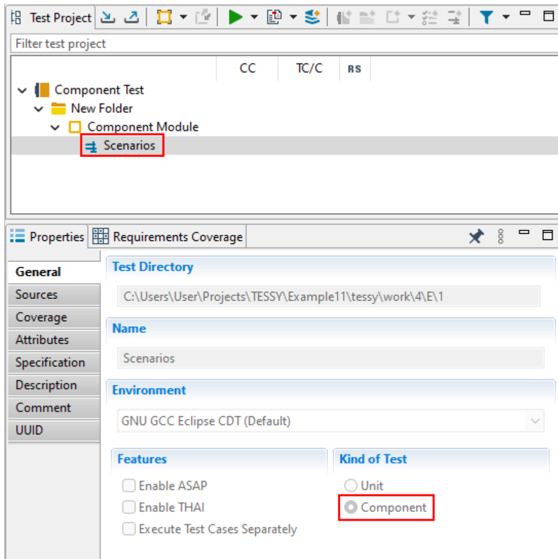
Figure 6.285: Scenarios of a component test
