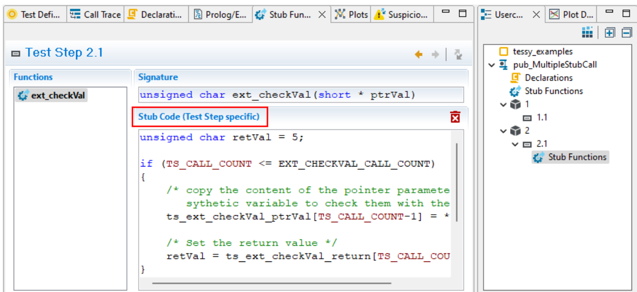
Figure 6.244: Usercode Outline view showing inserted stub code
