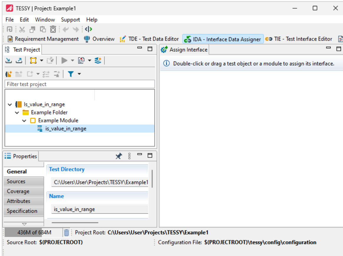
Figure 6.280: IDA perspective
