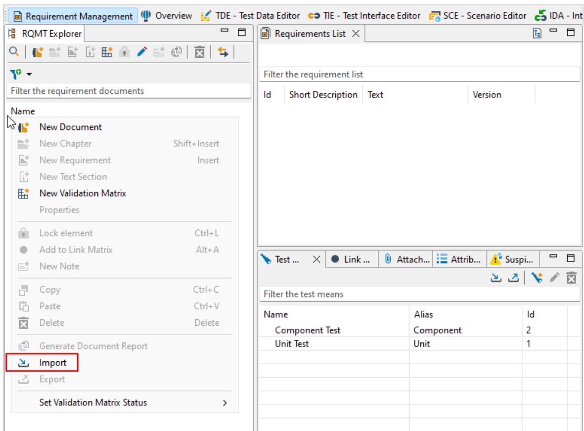
Figure 6.97: Importing requirements
