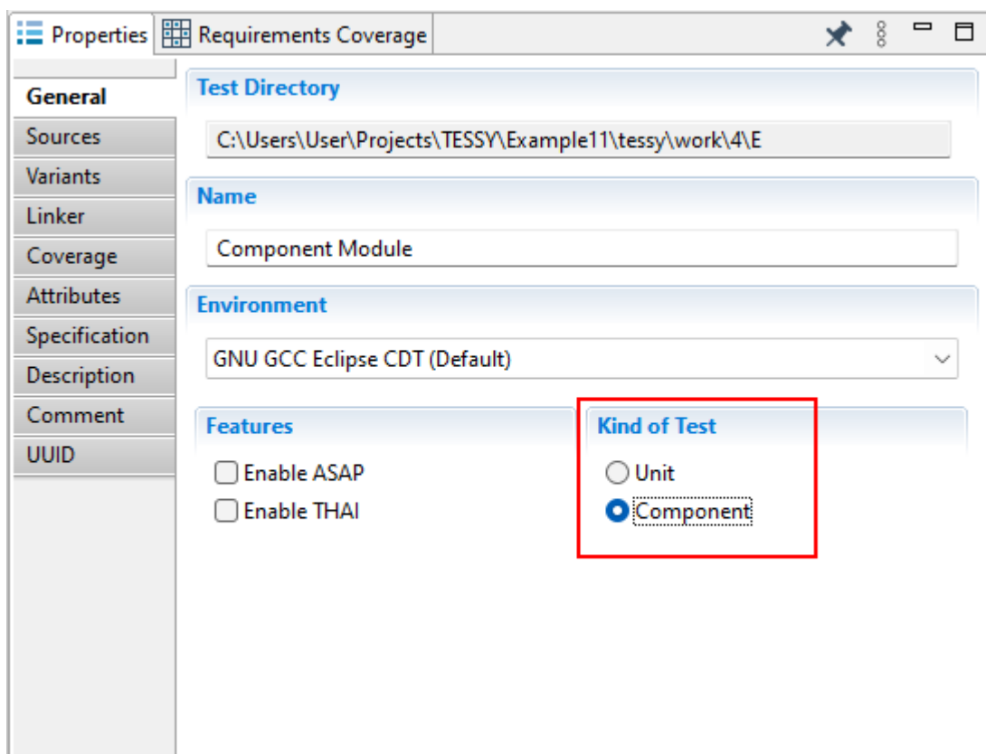
Figure 6.284: Component test
