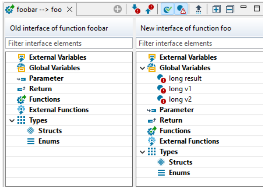
Figure 6.281: Compare view
