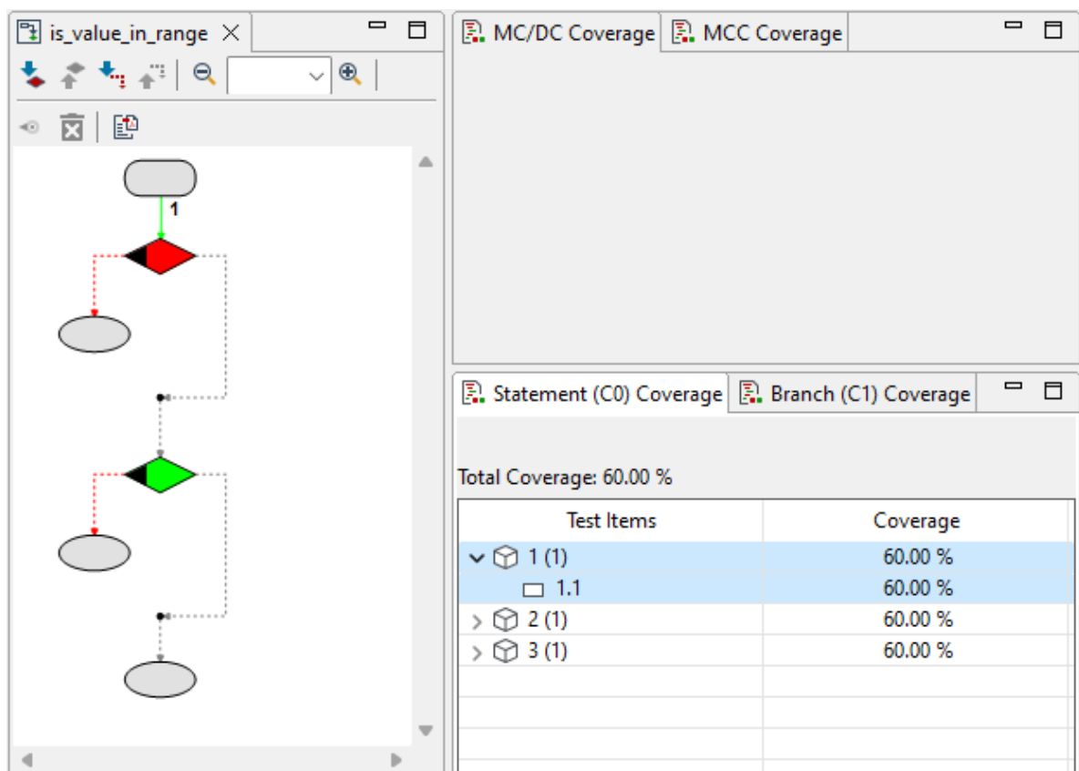
Figure 6.270: Statement coverage
