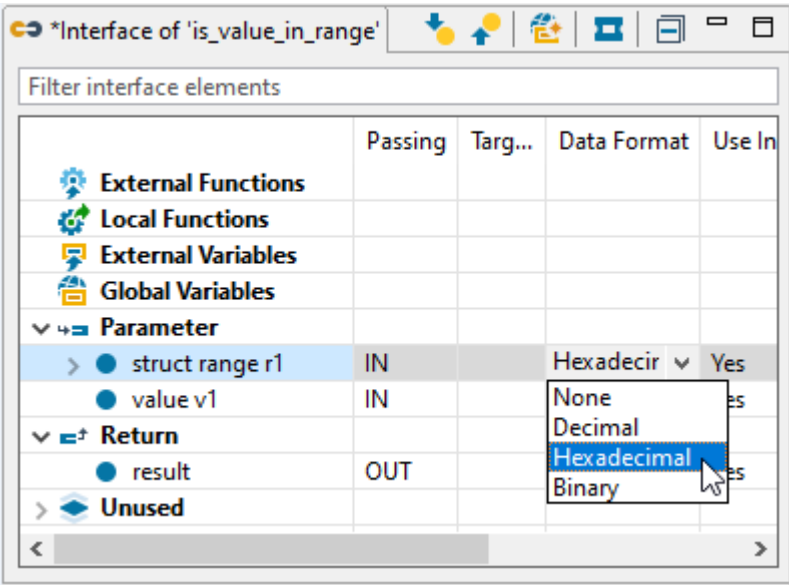
Figure 6.155: Setting the data format
