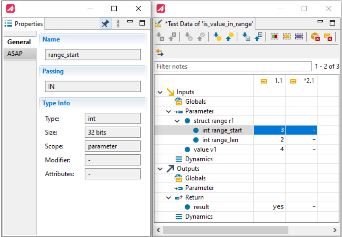
Figure 6.206: Type information of the variable long range_start
