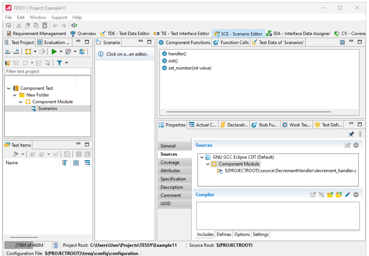
Figure 6.283: Perspective SCE - Scenario Editor
