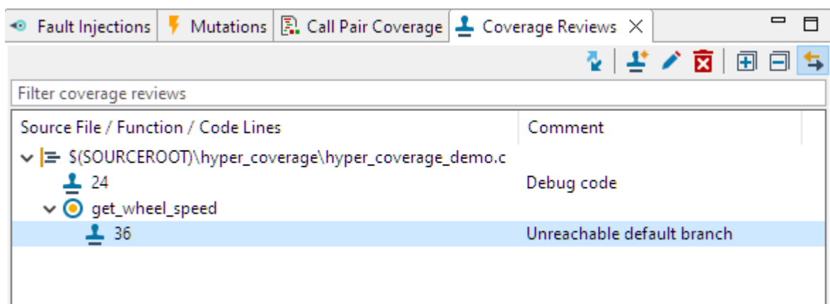
Figure 6.275: The new Coverage Reviews view
