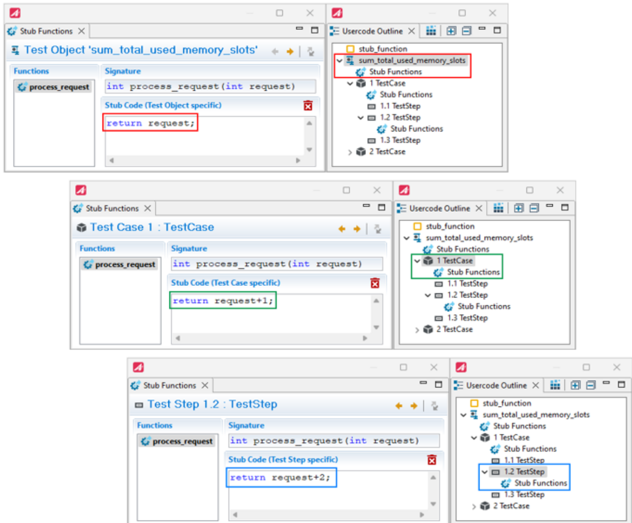
Figure 6.240: Stub code examples on test object, test case and test step level
