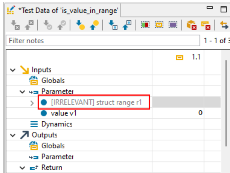
Figure 6.216: Passing direction set to irrelevant
