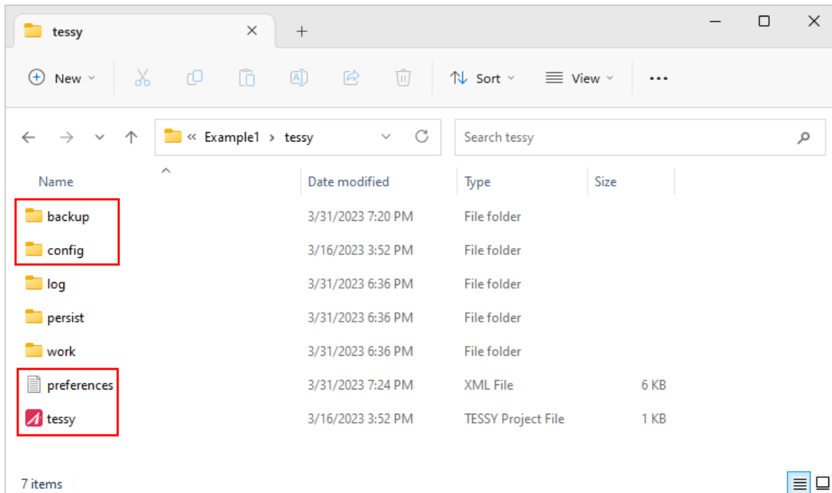
Figure 6.310: Directories and files within the database directory of the TESSY project
