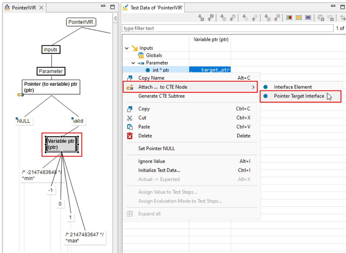
Figure 6.197: Attaching a pointer target to a CTE node
