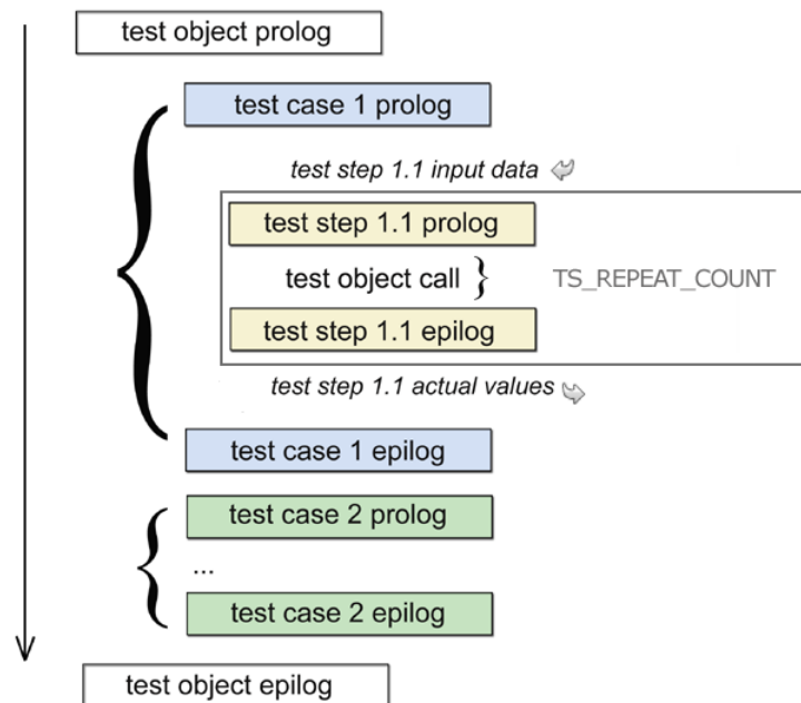
Figure 6.227: Call sequence of the usercode parts
