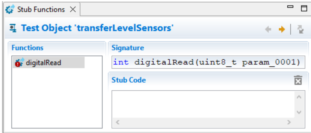
Figure 6.235: Stub Functions view without contents
