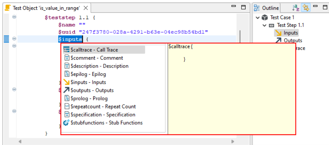
Figure 6.248: Script Editor menu with auto completions
