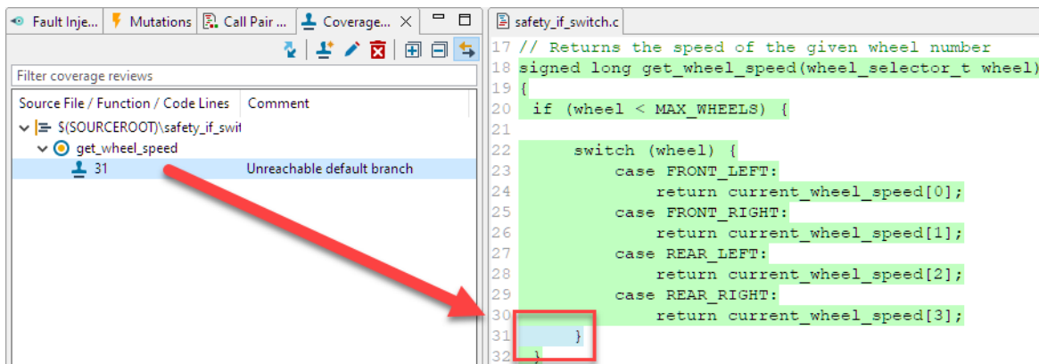
Figure 6.278: Added coverage highlighted blue
