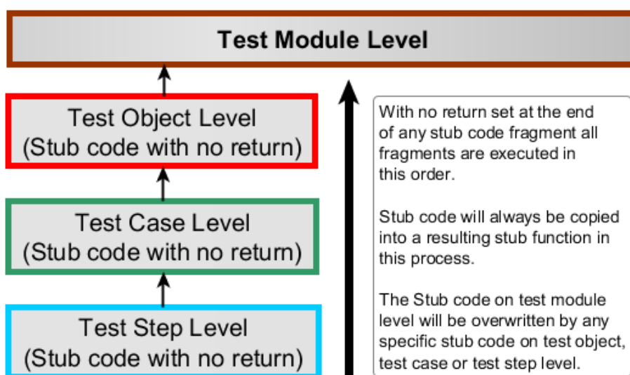
Figure 6.236: Test execution direction using stub code
