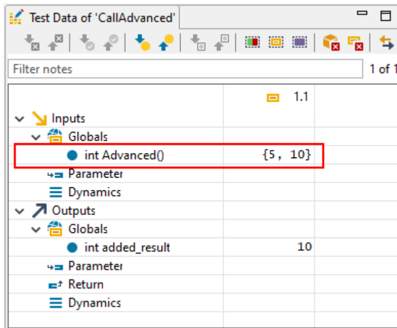
Figure 6.214: Entering values as vector for an advanced stub
