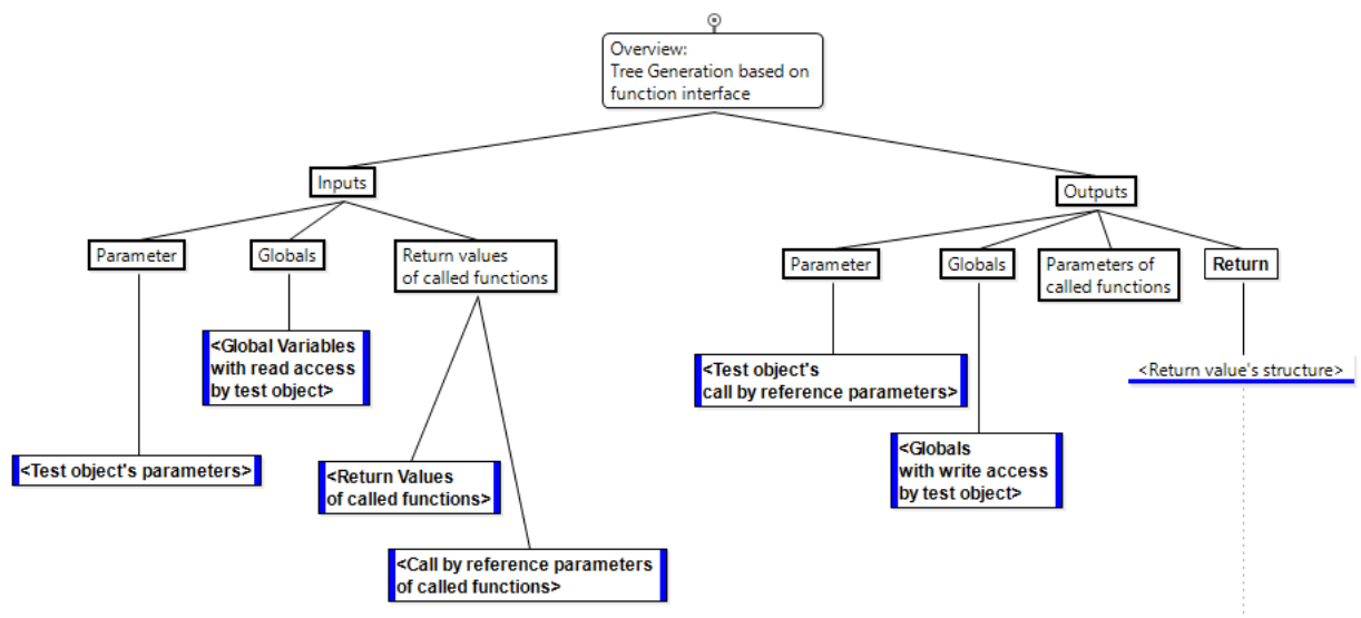
Figure 6.179: An overview on the automated tree generation based on the function interface
