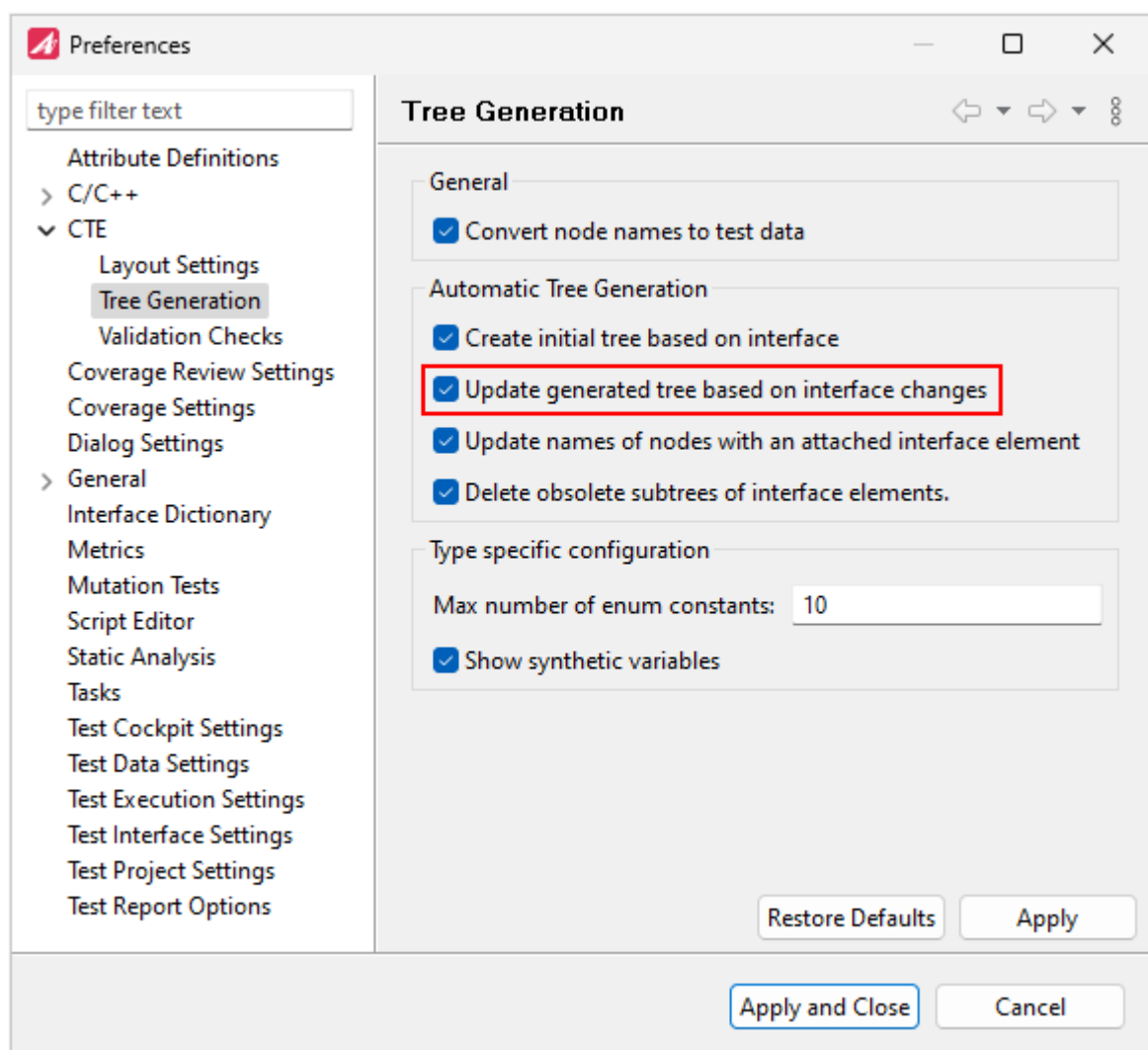
Figure 6.184: Settings in the CTE preferences
