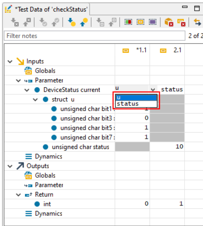
Figure 6.210: Clicking in the cell shows a combo box with the union components
