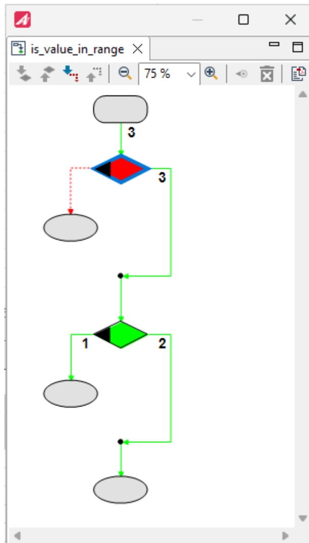
Figure 6.266: Flow Chart view
