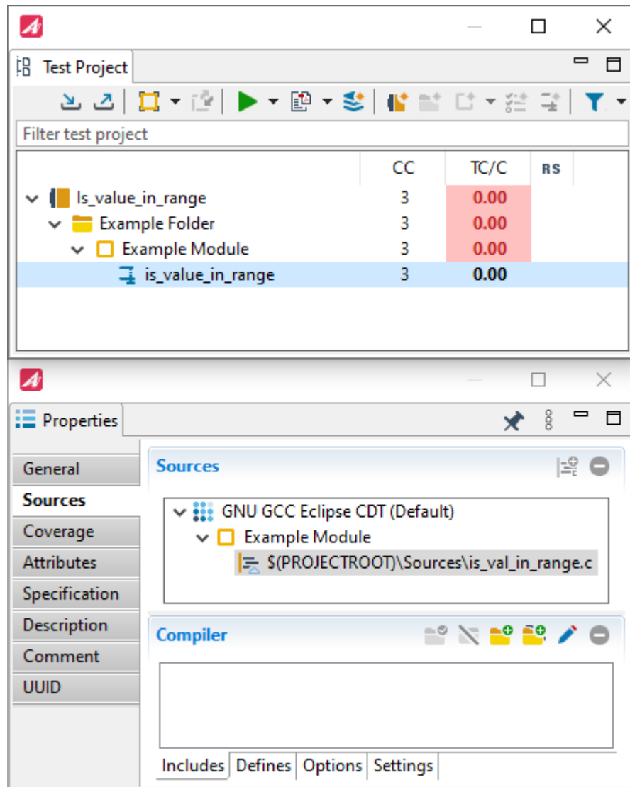
Figure 5.9: The function of the C-source is displayed as child of the module.
