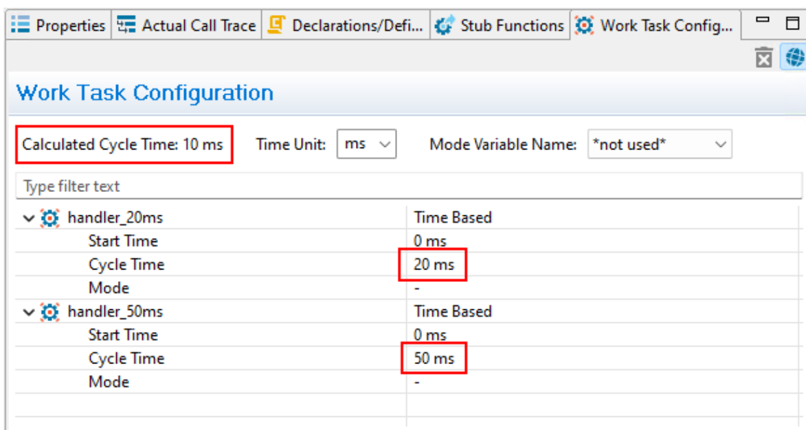
Figure 6.289: Calculated cycle time
