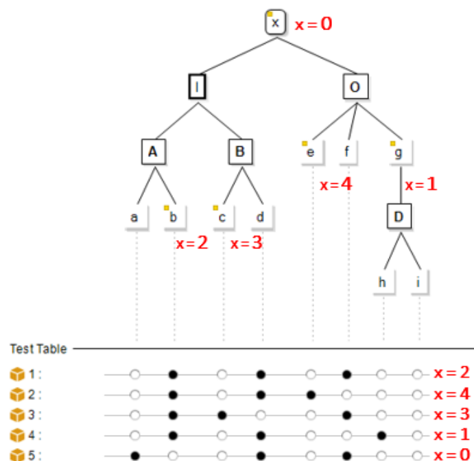
Figure 6.190: Variable assignments in classification trees
