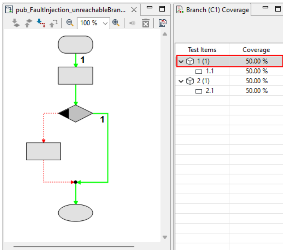
Figure 6.268: Condition view showing the sub flow coverage for one test case
