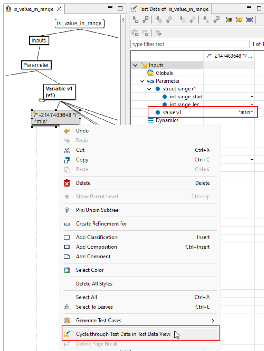
Figure 6.191: Start the cycling process in the tree area
