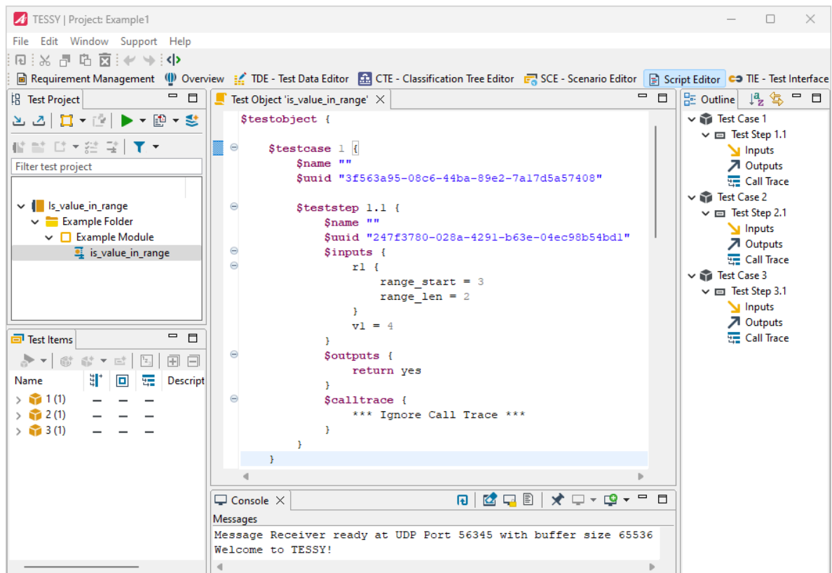
Figure 6.246: The Script Editor view
