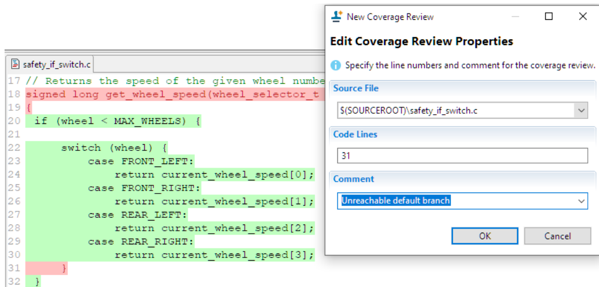
Figure 6.277: Adding new coverage reviews
