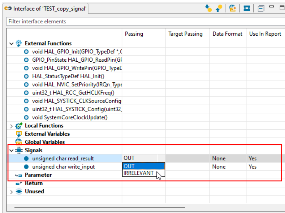
Figure 6.148: Required THAI attributes in the TIE
