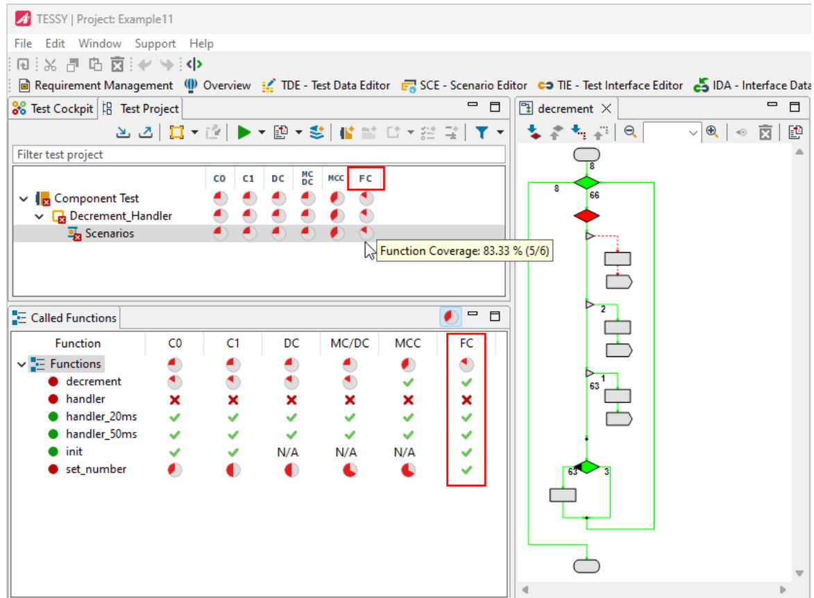
Figure 6.263: Coverage results within the CV perspective (component testing)
