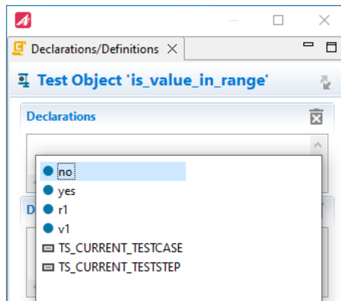
Figure 6.225: Declarations/Definitions view
