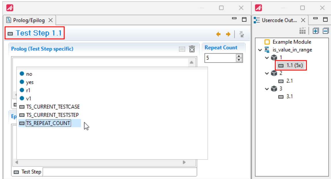
Figure 6.230: Prolog/Epilog functions
