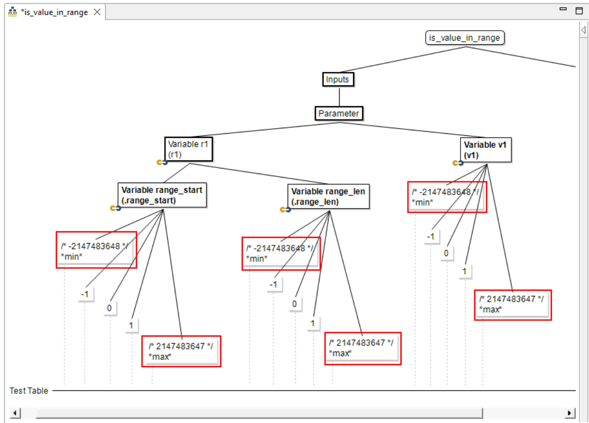
Figure 5.59: Deleting elements
