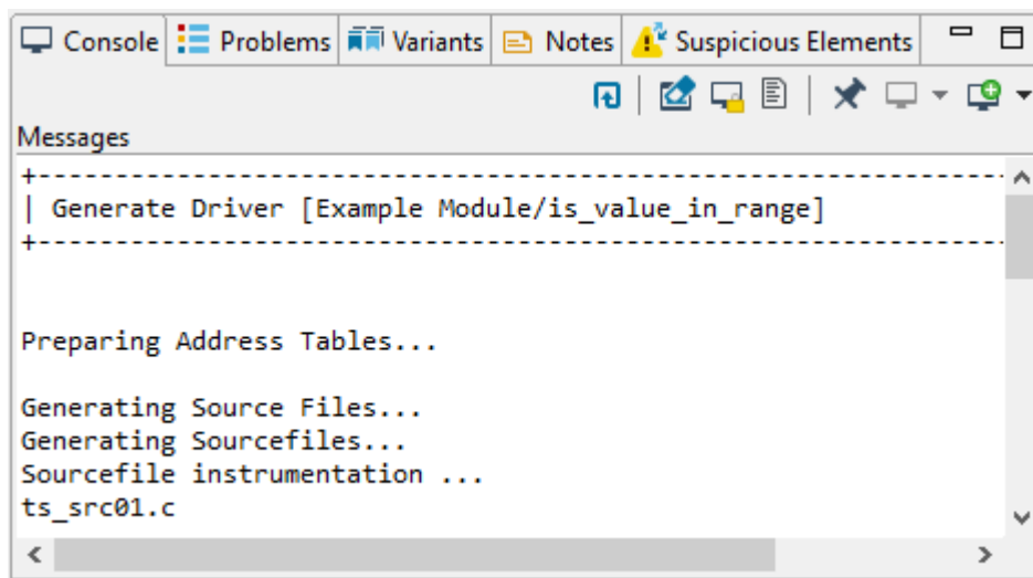
Figure 6.78: Console view
