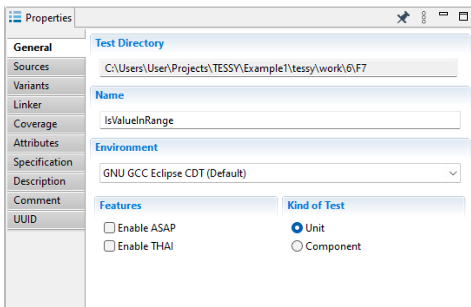
Figure 6.61: Properties view
