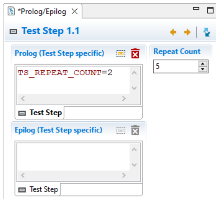
Figure 6.226: Prolog/Epilog view
