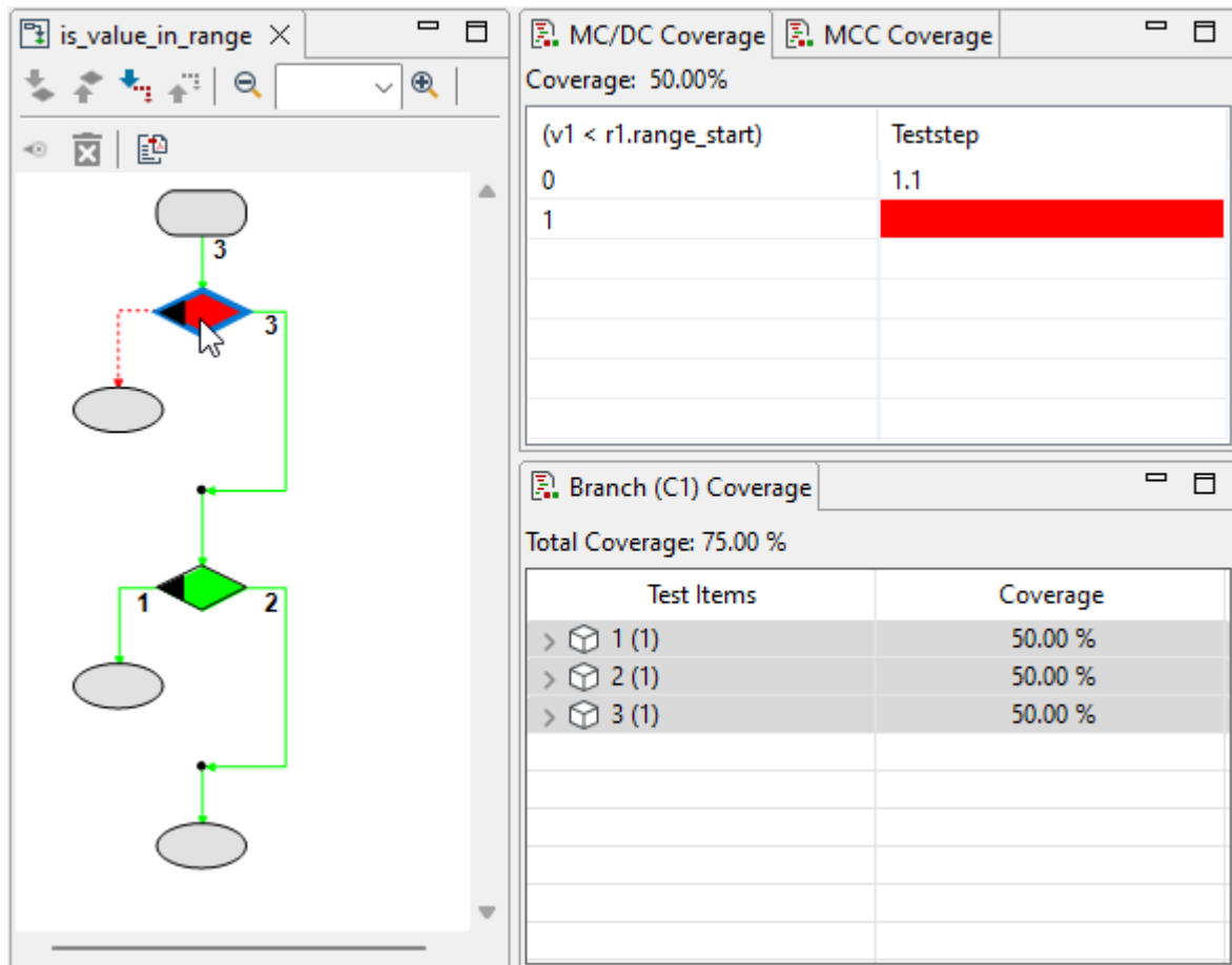
Figure 6.273: MC/DC coverage
