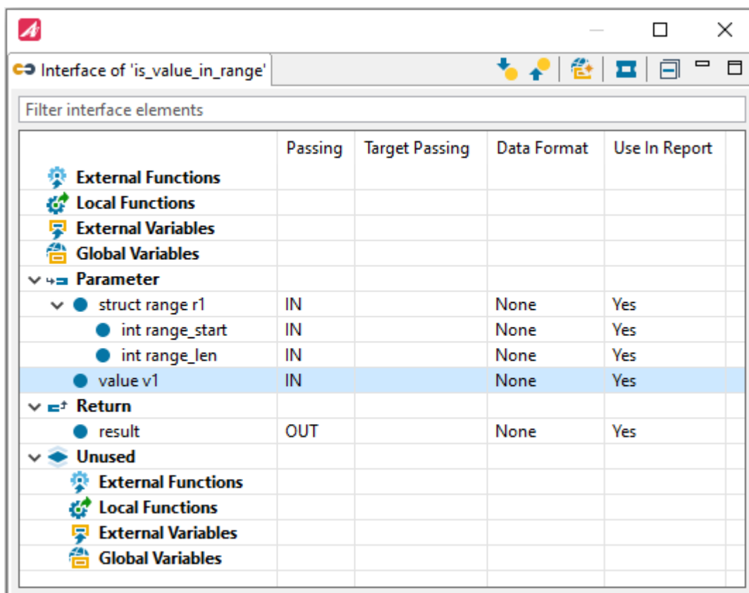
Figure 6.152: Interface view
