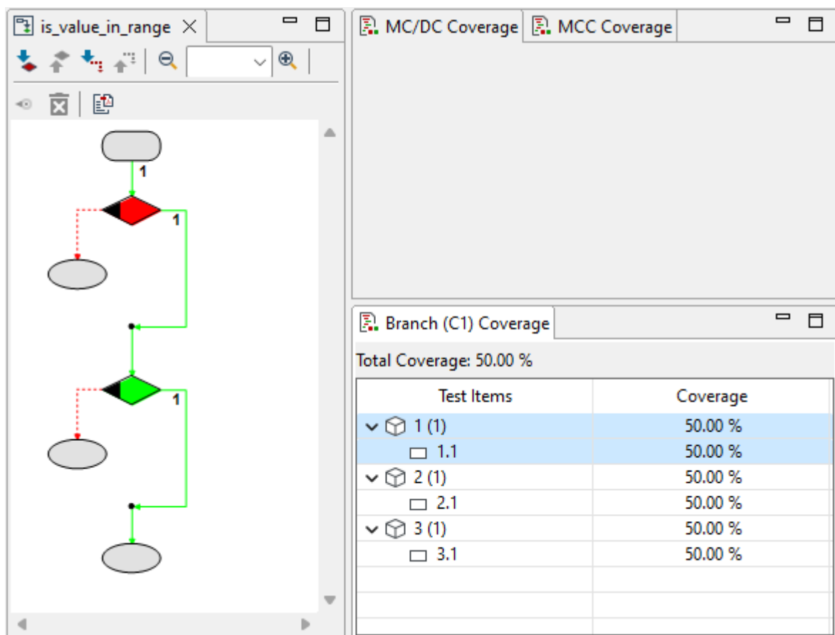
Figure 6.271: Branch coverage
