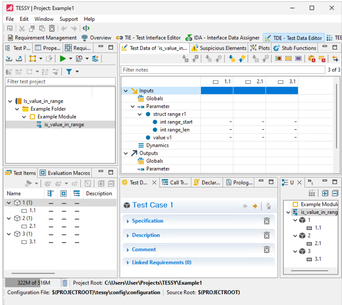
Figure 6.205: TDE perspective
