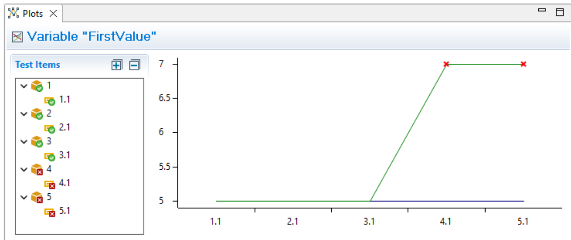
Figure 6.245: Plots view
