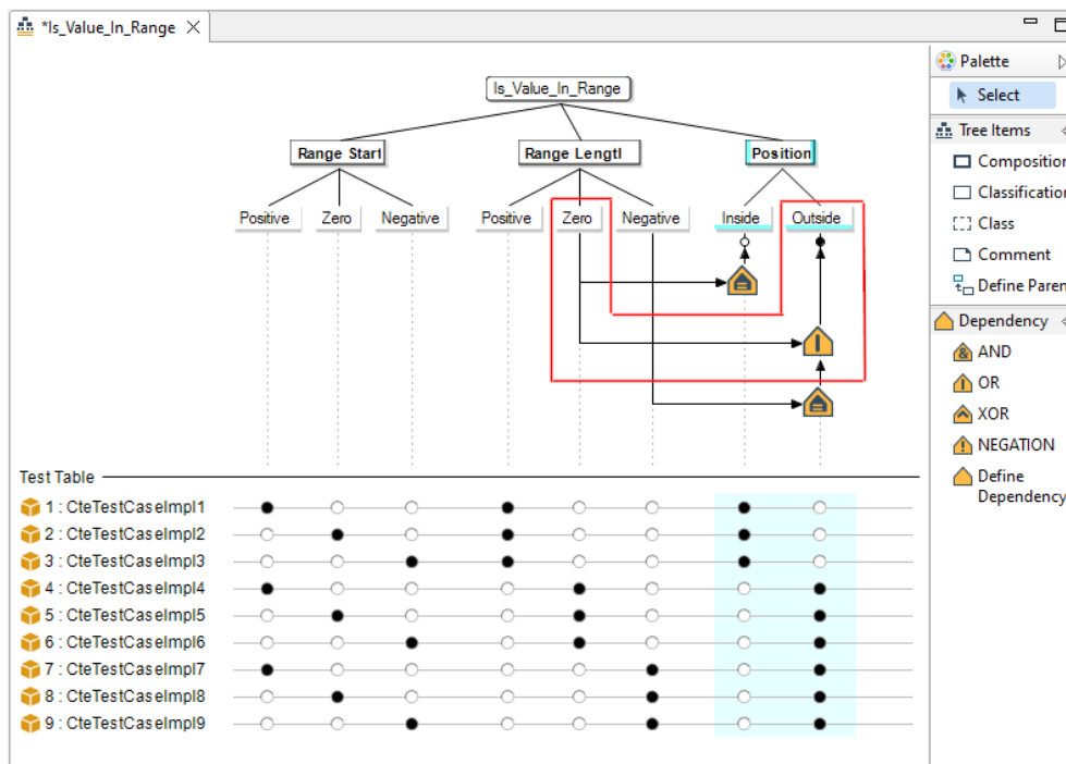
Figure 6.203: Composite dependency
