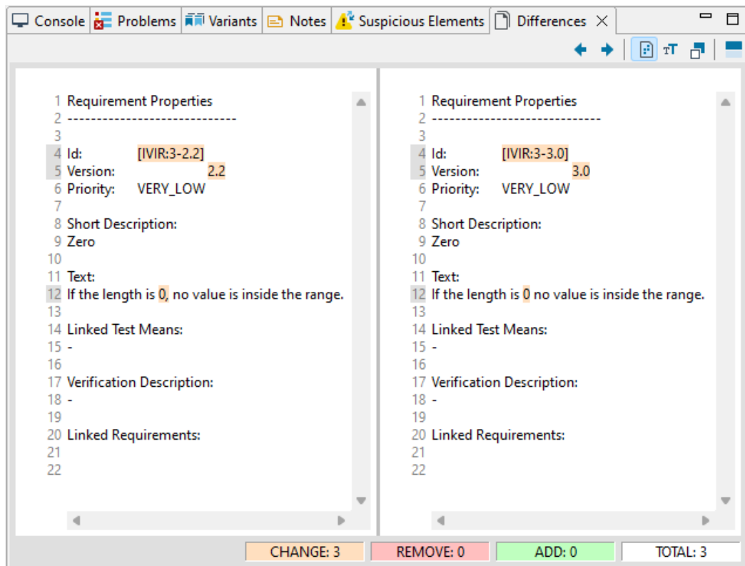
Figure 6.127: Differences view
