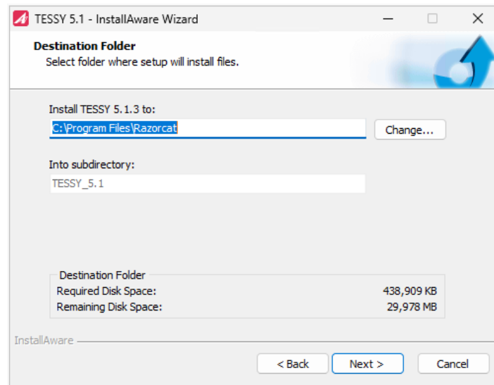
Figure 1.2: Destination Folder
