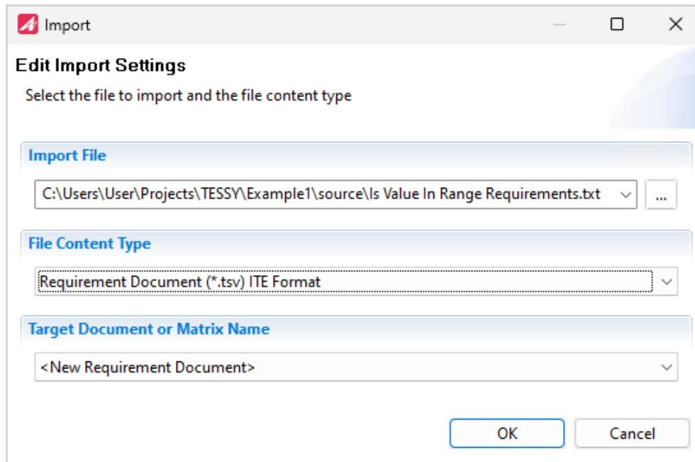
Figure 5.30: Import dialog
