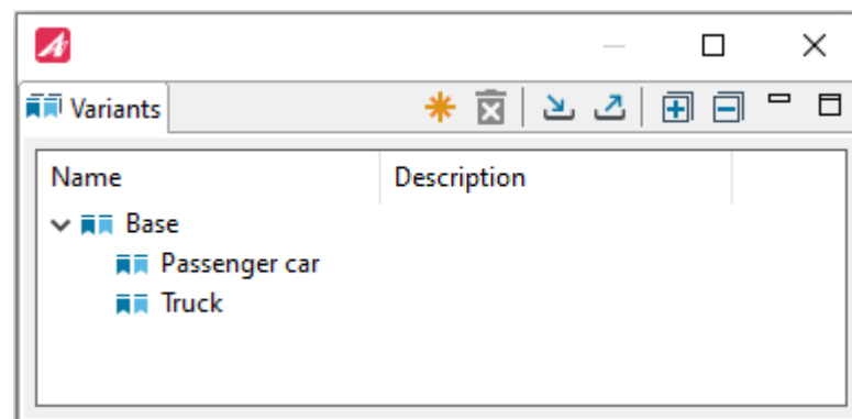
Figure 6.81: Variants View
