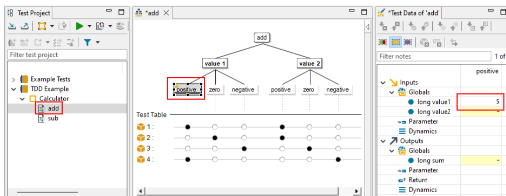
Figure 5.101: Creating test cases for TDD
