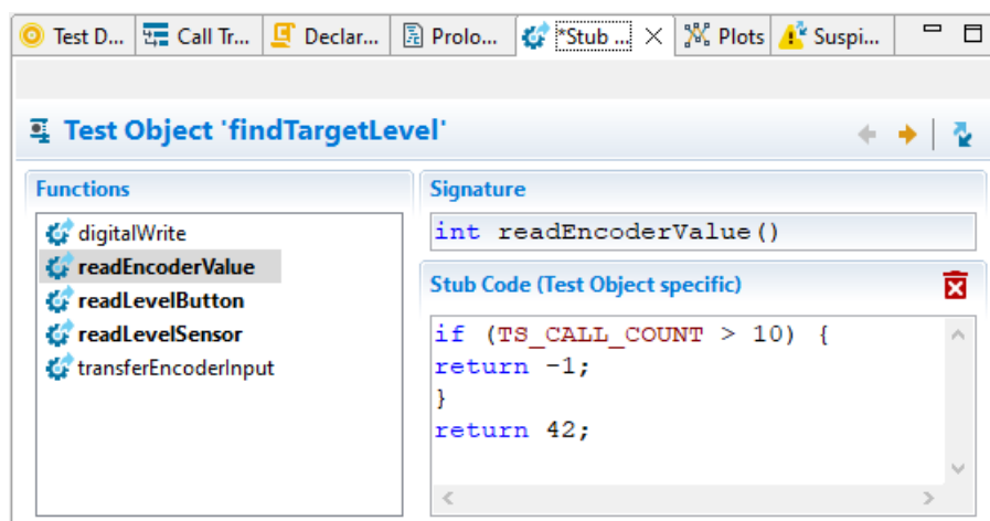
Figure 6.238: Stub Functions view with code using TS_CALL_COUNT macro
