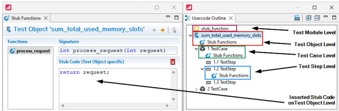
Figure 6.239: Stub Code Levels in the Usercode Outline view
