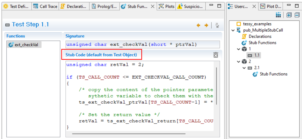
Figure 6.243: Usercode Outline view showing inherited stub code
