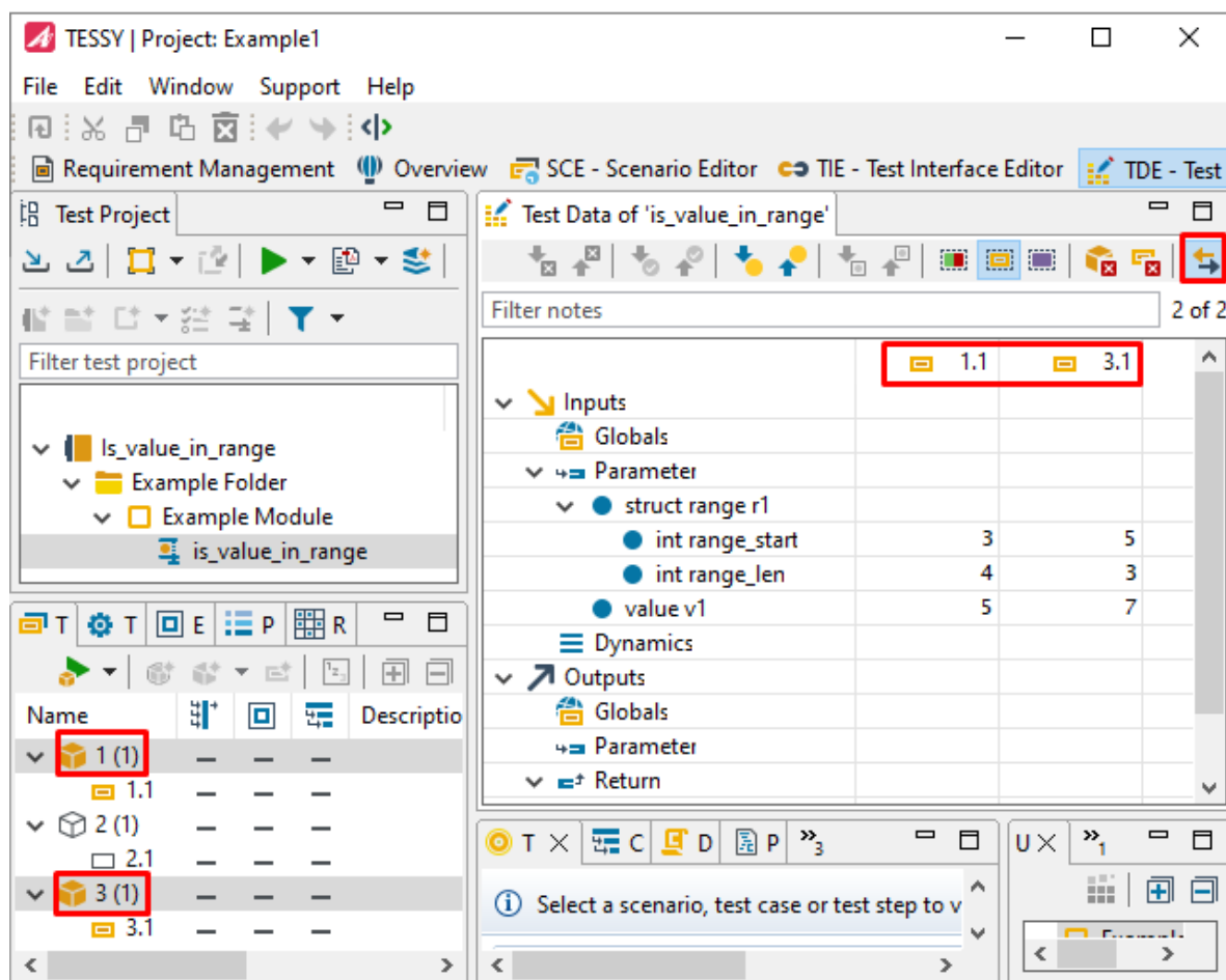
Figure 6.209: Test Data view showing selected test steps.
