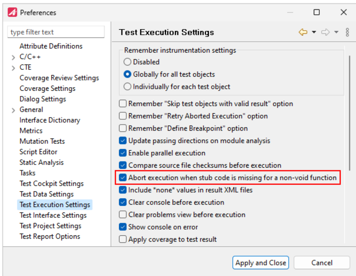
Figure 6.237: TESSY Preferences: Abort on missing stub code
