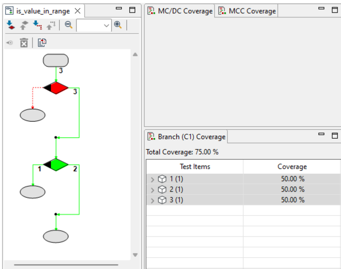
Figure 6.272: MC/DC Coverage view
