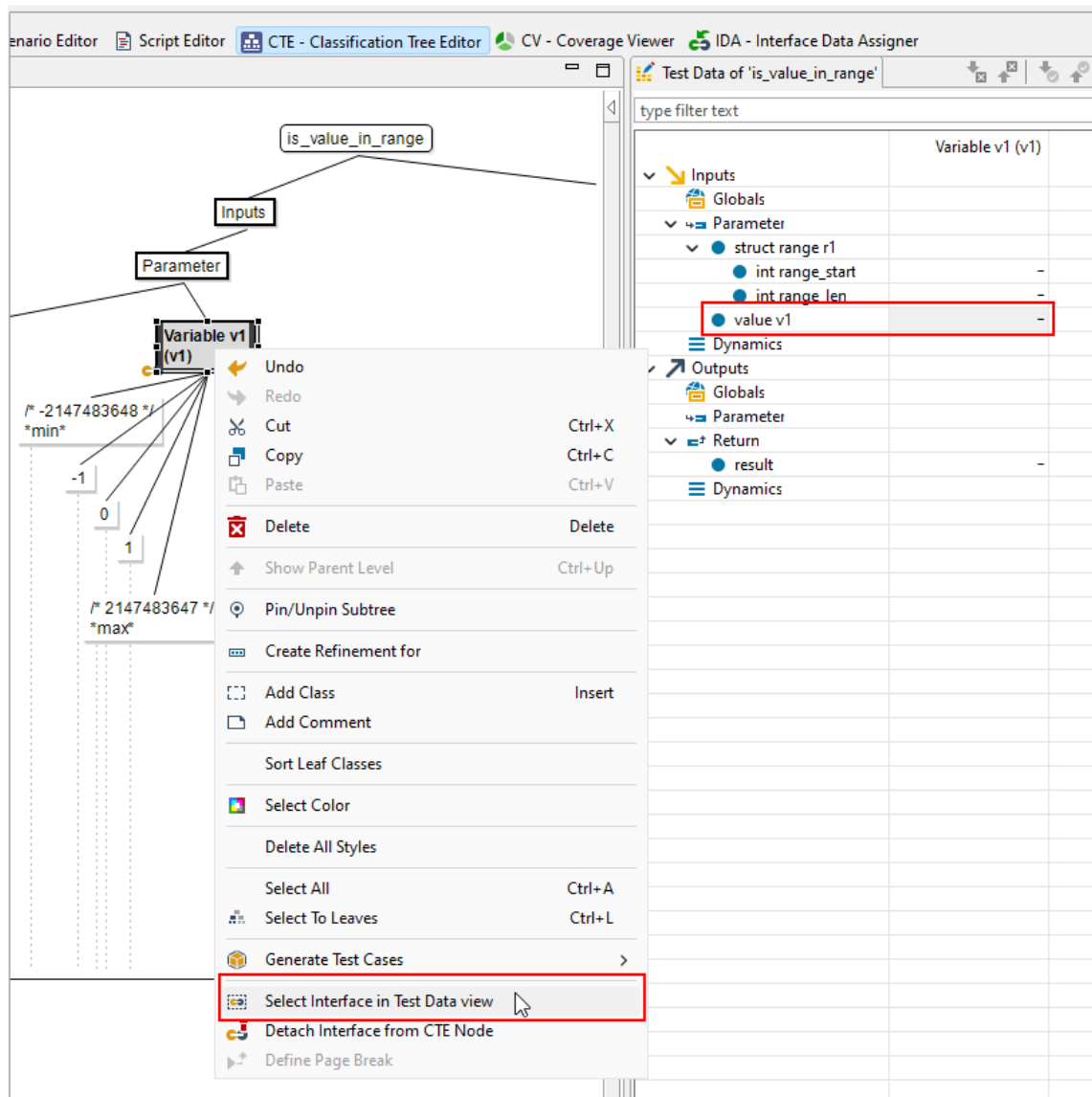
Figure 6.193: Select interface in Test Data view
