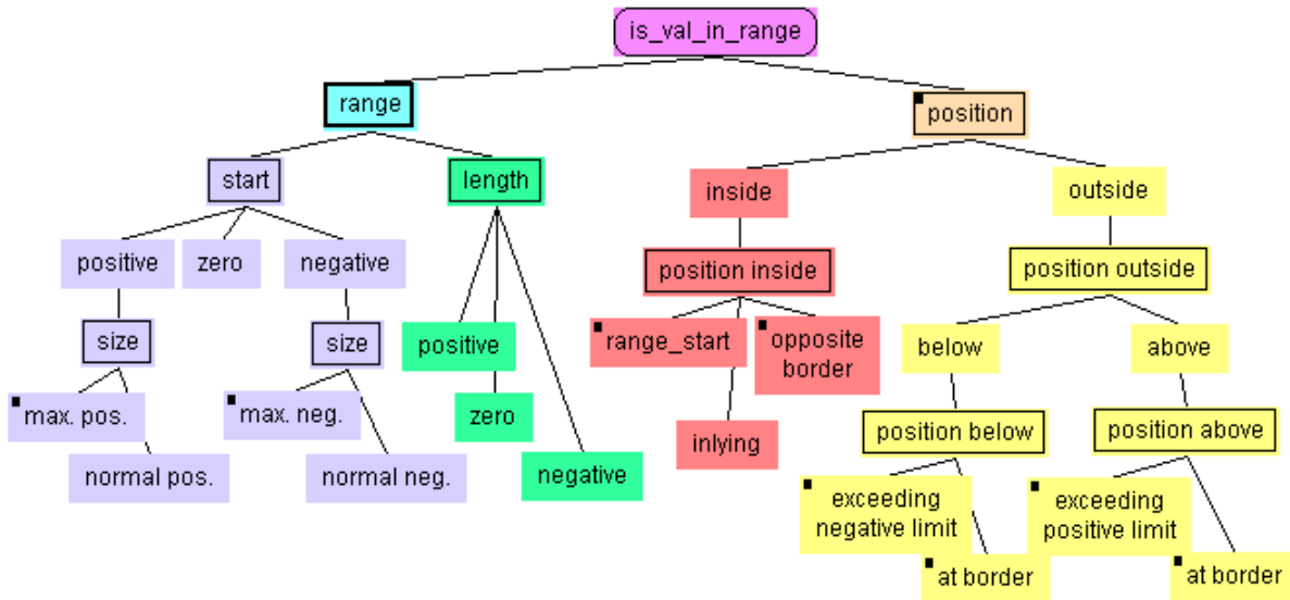
Fig. 14: The completed classification tree
