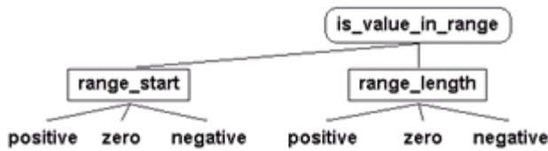
Fig. 8: The classification tree for "is_value_in_range" - further developed
