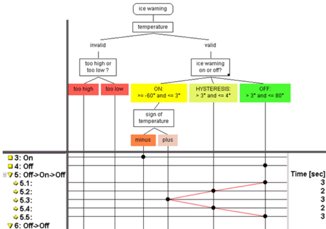
Fig. 32: Hysteresis using a sequence
